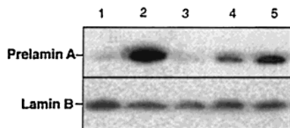
Figure 3. Inhibition of FT by 1 in human lung cancer cells (lane 1: treated with vehicle; lane 2: treated with a known potent, cell-permeable FTI, B581, 62 at 100 \mu M; lanes 3, 4, and 5: treated with 1 at 100, 200, and 500 \mu M, respectively).
